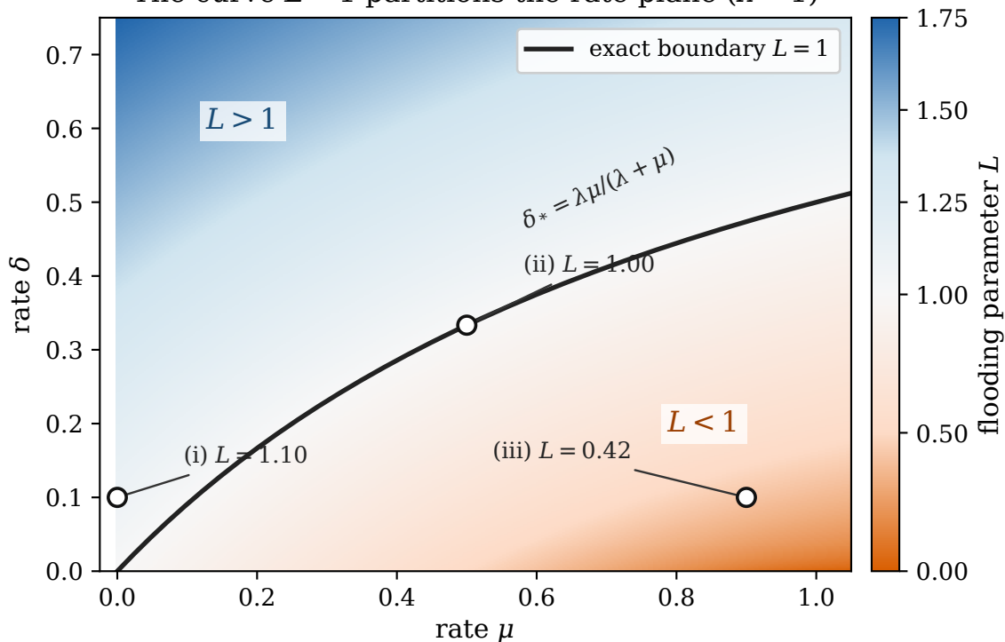
The curve L = 1 partitions the rate plane ( \lambda = 1 )
